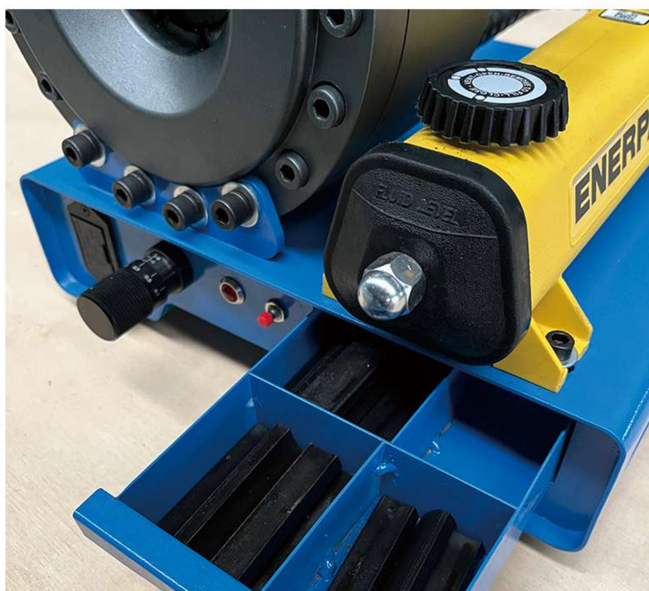
DIE STORAGE DEVICE
